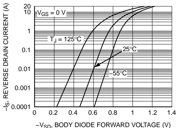
Figure 6. Diode Forward Voltage Variation with Source Current and Temperature
