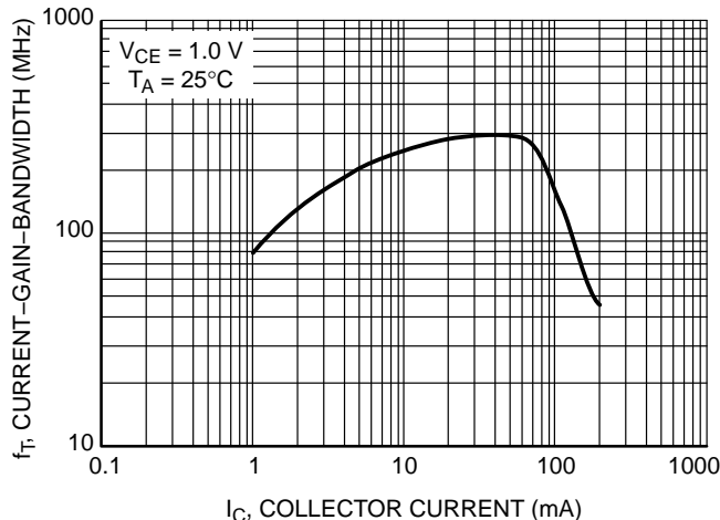
Figure 22. Current-Gain-Bandwidth Product
