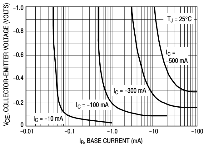
Figure 22. Saturation Region
