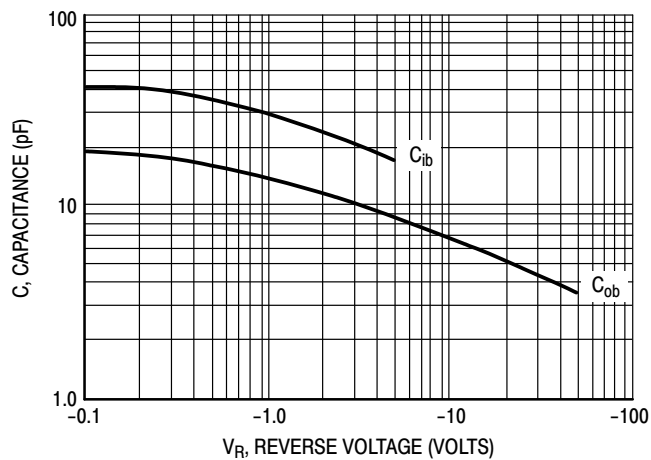
Figure 24. Capacitances
