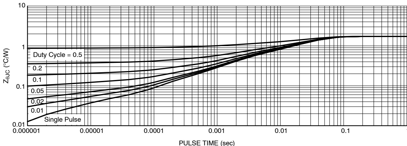
Figure 13. Thermal Impedance
