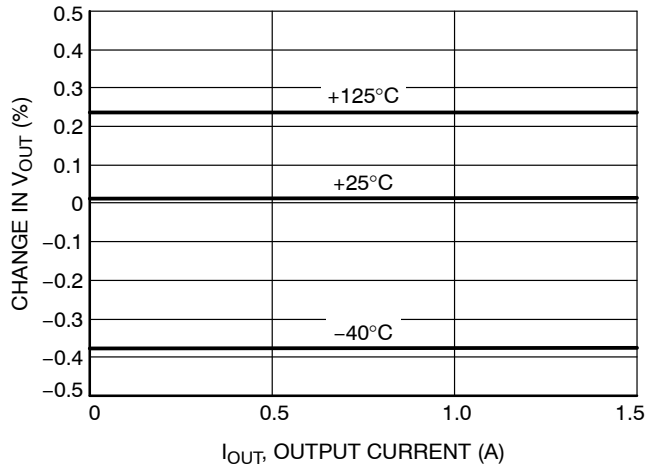
Figure 6. Load Regulation
