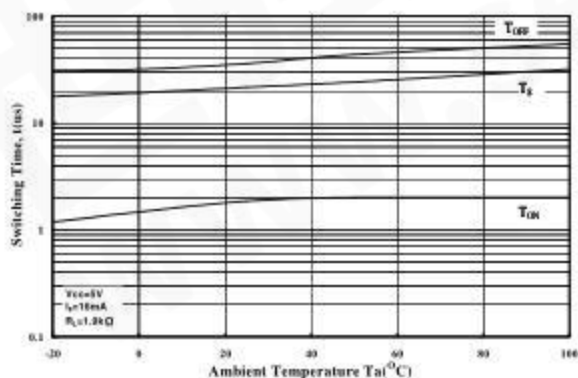
Figure 17. Switching Time vs. Ambient Temperature
