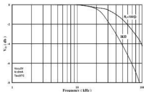
Figure 18. Frequency Response
