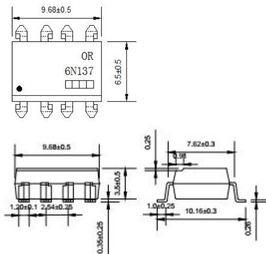
( 3 ) OR-6N137S
