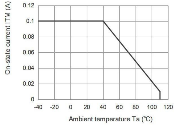
Fig.2 On-state current ITM (A) vs. Ambient temperature
