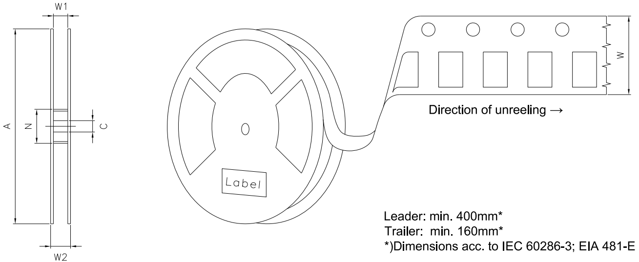
Reel dimensions in mm (inch)
