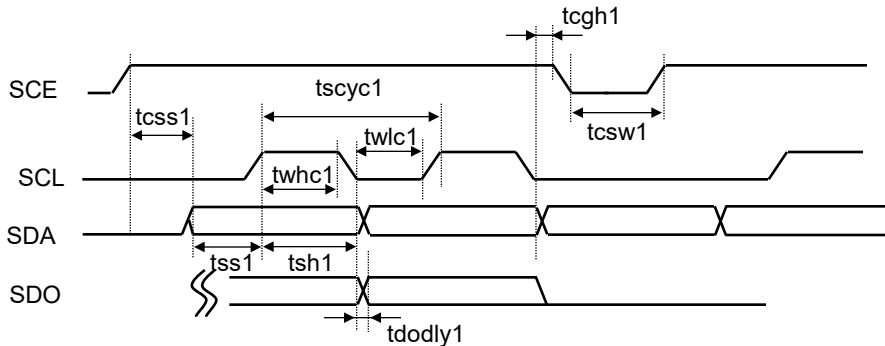
Interface timing chart
