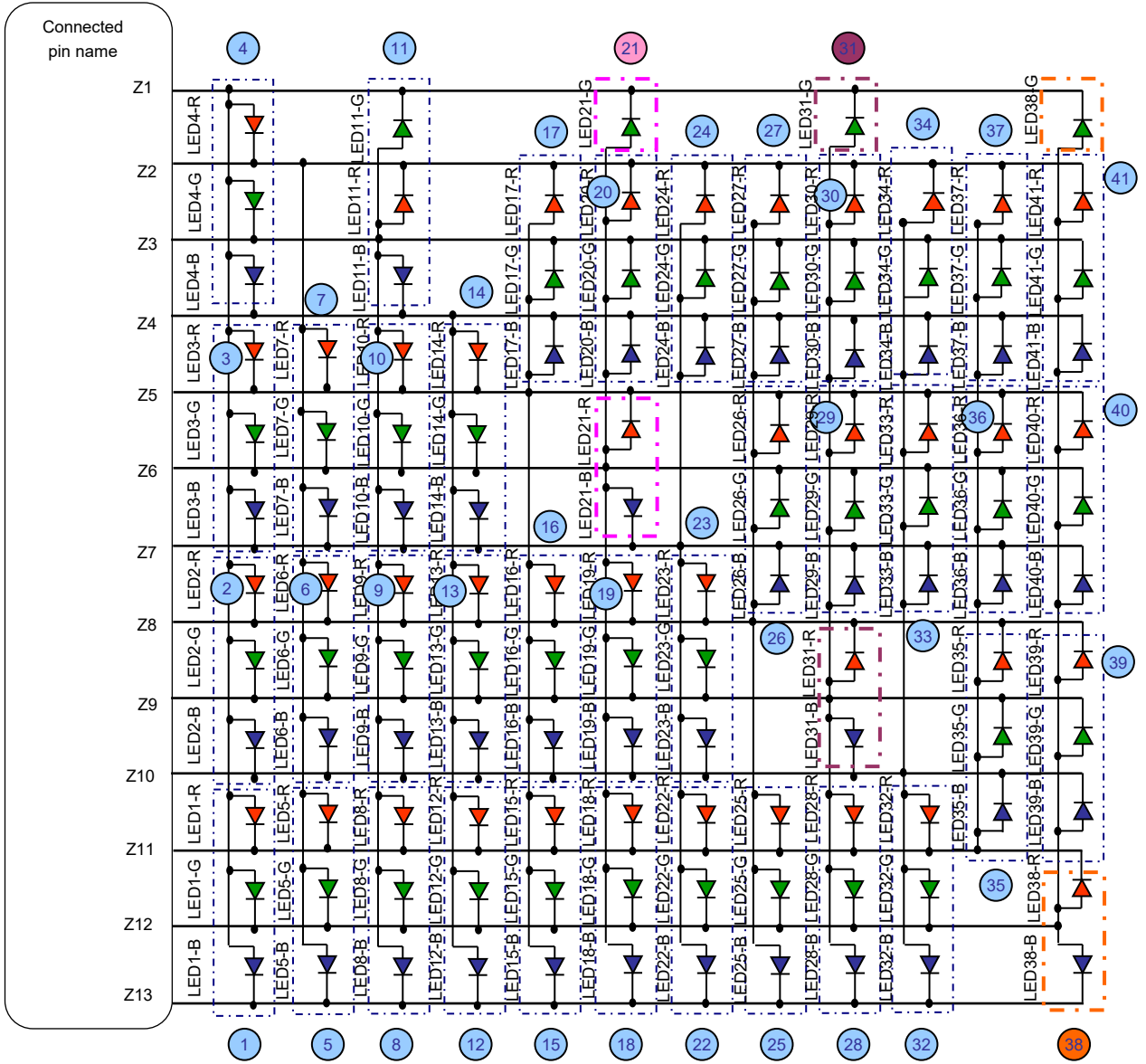
Example of RGB LED connection
