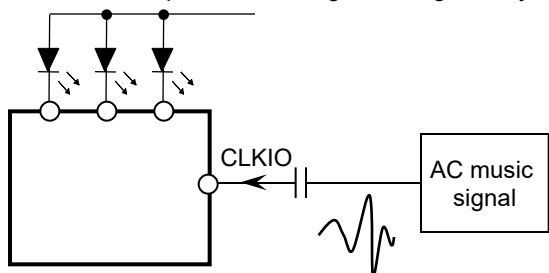
CLKIO uses as music input when melody mode is enabled by register MTXMODE [1:0].
