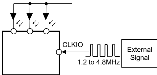
CLKIO uses as external input by using EXTCLK register
