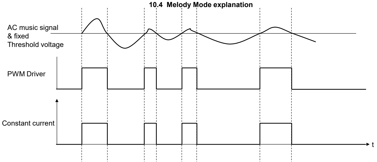
Example of Fixed threshold mode
