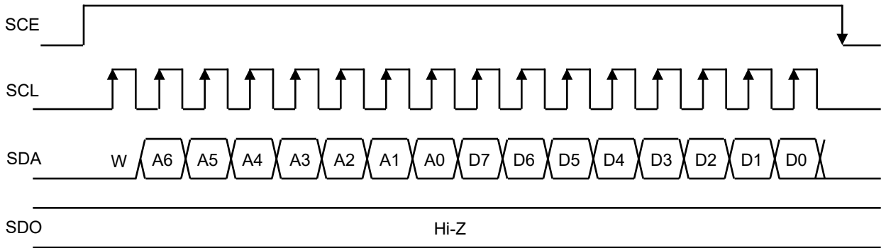
Writing access timing
