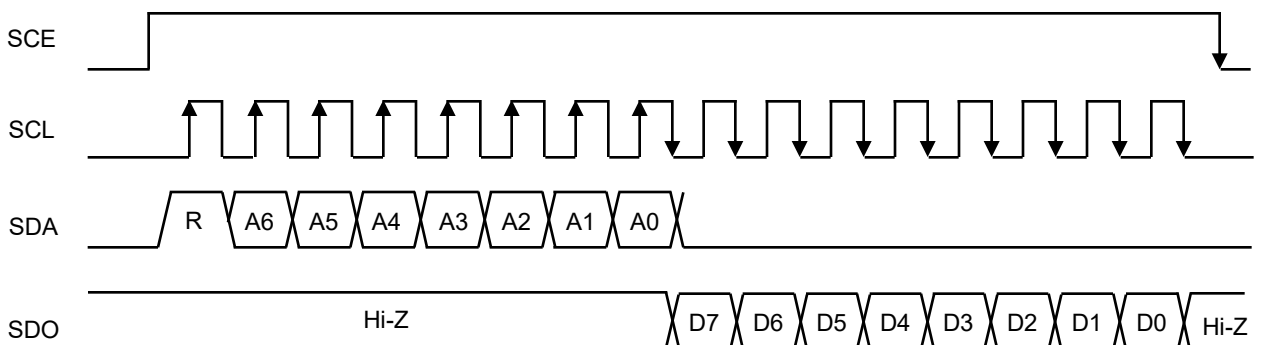
Read access timing
