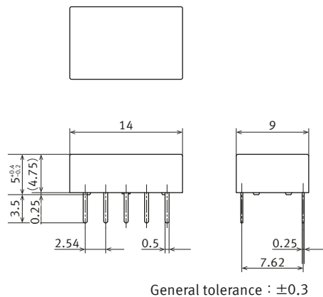
External dimensions PC board terminal ( standard )
