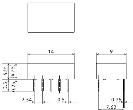
External dimensions PC board terminal (standard)
