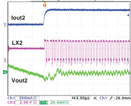
DC-DC2 Iout2 = 10 mA to 250 mA , Δt = 1 μsec
