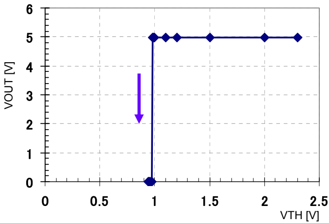
Figure B-8 Output Voltage vs VTH
