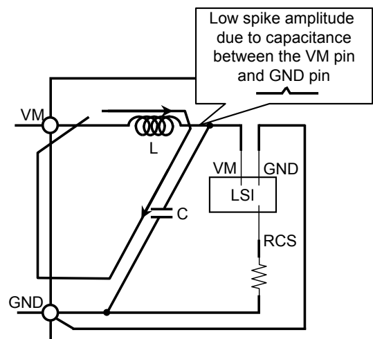
Figure 3. Recommended pattern
