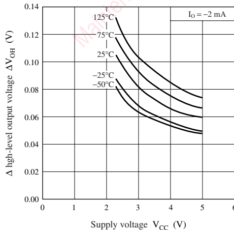
\Delta high-level output voltage — Supply voltage
