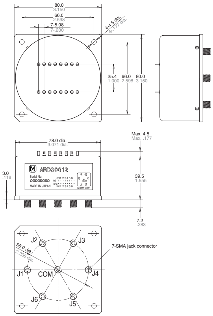
Latching type
