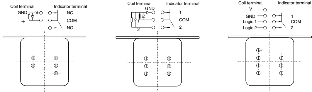
Latching with TTL driver (with self cut-off function)
