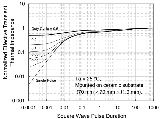
Thermal Response
