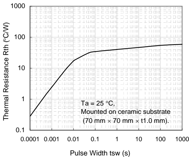
Rth - tsw
