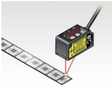
Checking for overlapped lead frames
