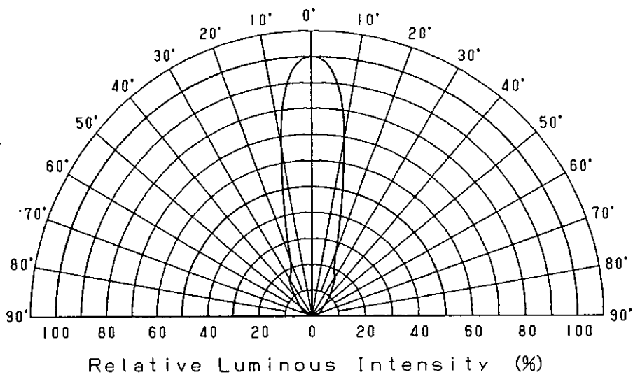
Directive Characteristics
