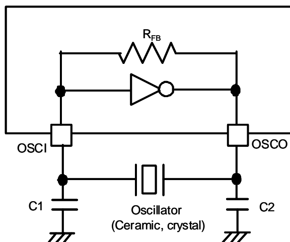
Figure:1.6.1 Oscillation Circuit
