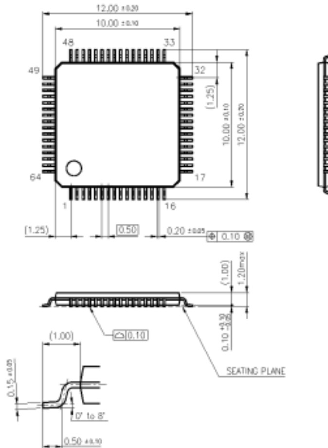
Figure:1.7.5 Package Dimension of 64 pin TQFP
