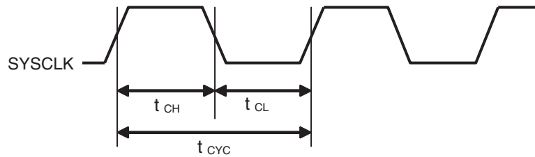
Figure:1.6.5 External Clock Timing
