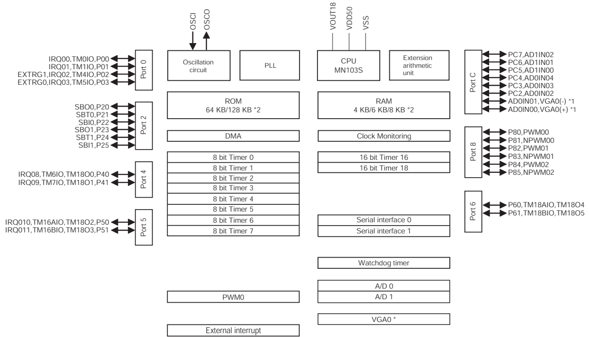
Figure:1.4.2 Block Diagram (MN103SFN0/N4 series)
