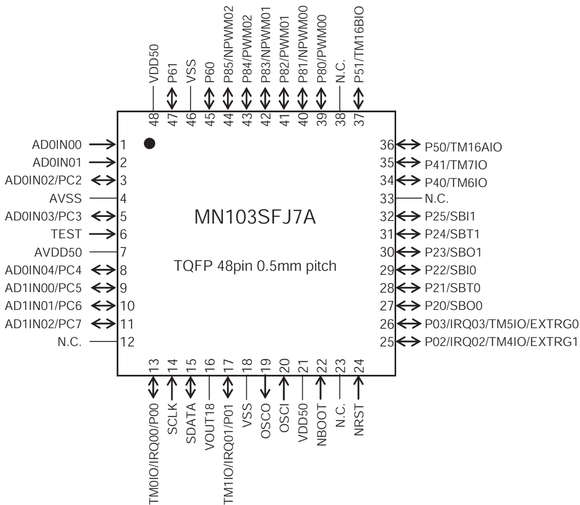
Figure:1.3.1 Pin Configuration (MN103SFJ7A)
