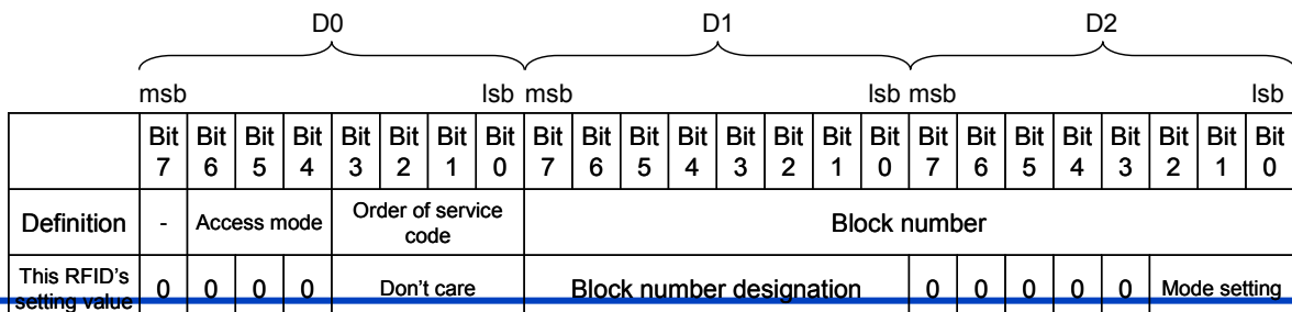
Figure 4-9 Block Element of 2 Bytes
