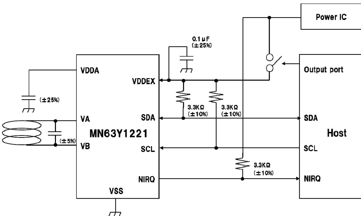
Figure 2-3 Connection Example
