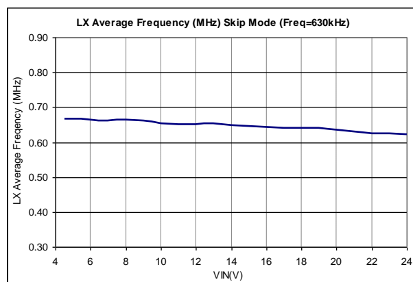
Frequency = 630 kHz
