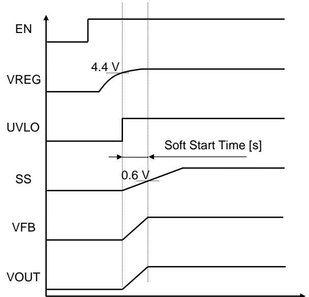
Figure : Soft Start Operation
