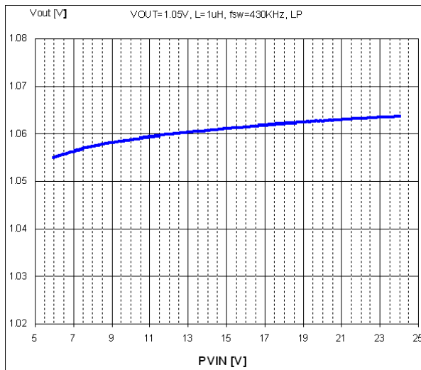
Frequency = 430 kHz
