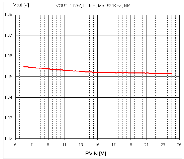
Frequency = 630 kHz
