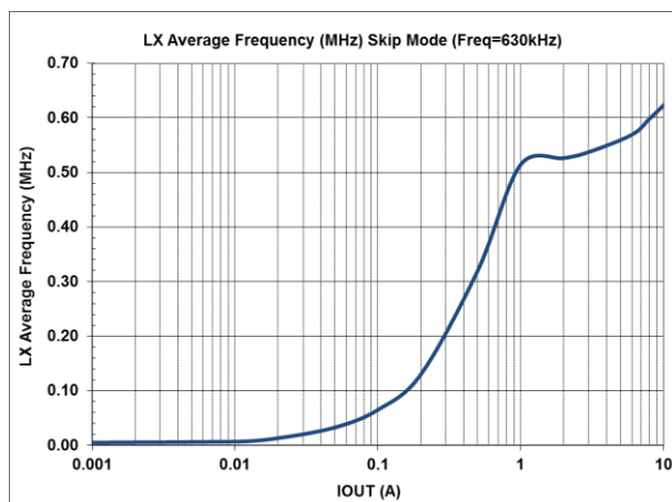
Frequency = 630 kHz
