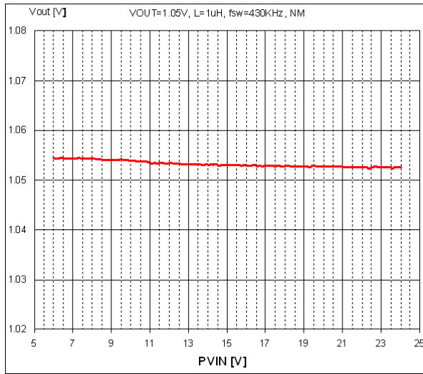
Frequency = 430 kHz
