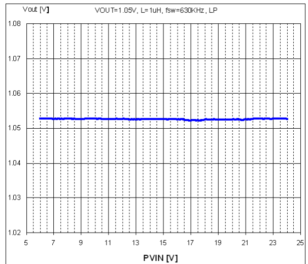
Frequency = 630 kHz
