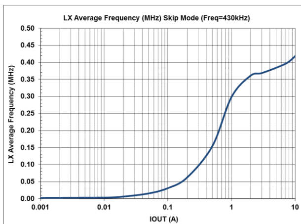
Frequency = 430 kHz
