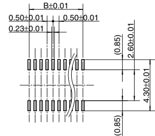
Recommended metal mask pattern Metal mask thickness: When 150 μm (Opening area ratio: 58%)
