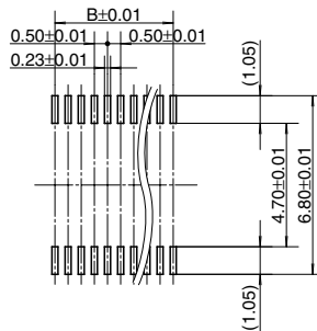
Recommended metal mask pattern Metal mask thickness: When 120 μm (Opening area ratio: 69%)
