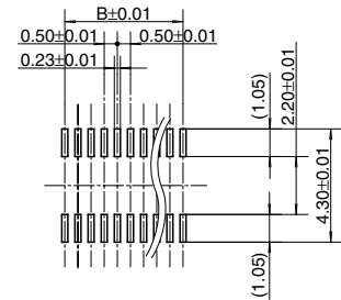
Recommended metal mask pattern Metal mask thickness: When 120 μm (Opening area ratio: 72%)
