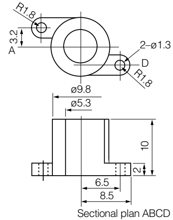
Sectional plan ABCD
