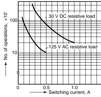
2. Life curve
