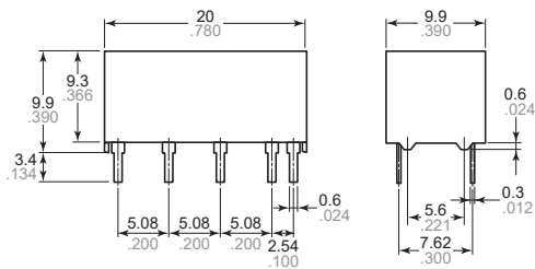
External dimensions
