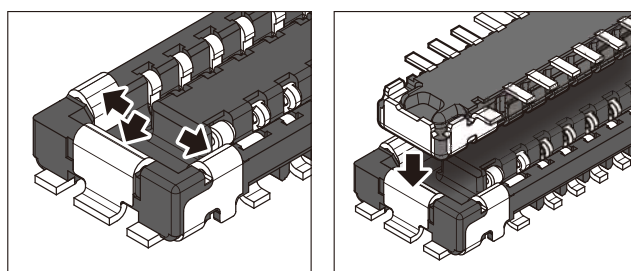
Flange section highly resistant to impact (in direction of arrow)!
