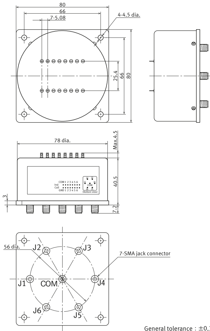
External dimensions
