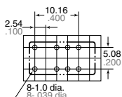
PC board pattern (Bottom view)
