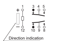
Schematic (Bottom view) Single side stable
