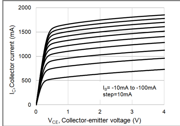
Fig.8 Collector Current
