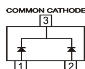
Fig. 16(TOP VIEW)
