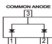
Fig. 15(TOP VIEW)
