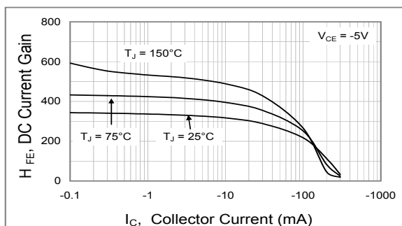
Fig.3 DC Current Gain
