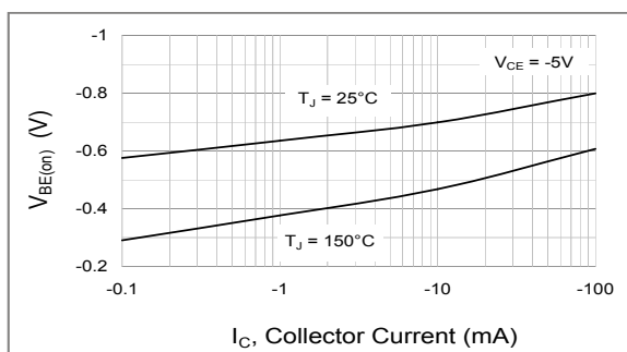
Fig.4 Base-Emitter Voltage
