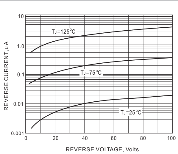
FIG. 2-TYPICAL REVERSE CHARACTERISTICS
