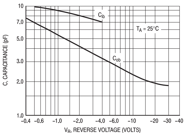
Figure 11 . Capacitances
