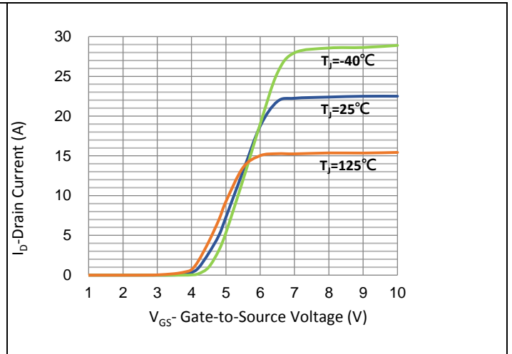
Fig.2 Transfer Characteristics
