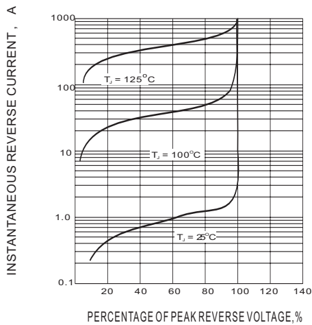
Fig. 3-TYPICAL REVERSE CHARACTERISTIC
