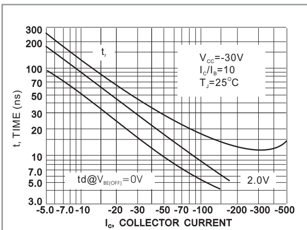
Fig.3-Turn-On Time
