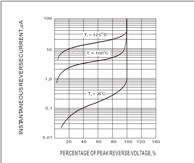
Fig.3-TYPICAL REVERSE CHARACTERISTIC
