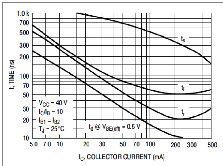
Fig.3 Switching Time
