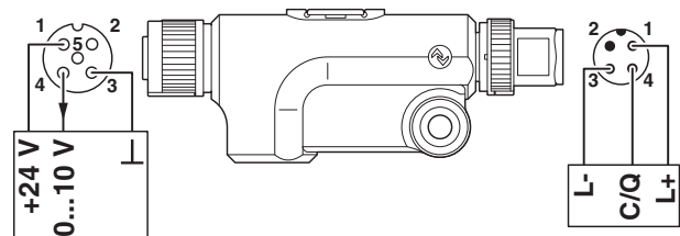
Figure 5 Connection example
