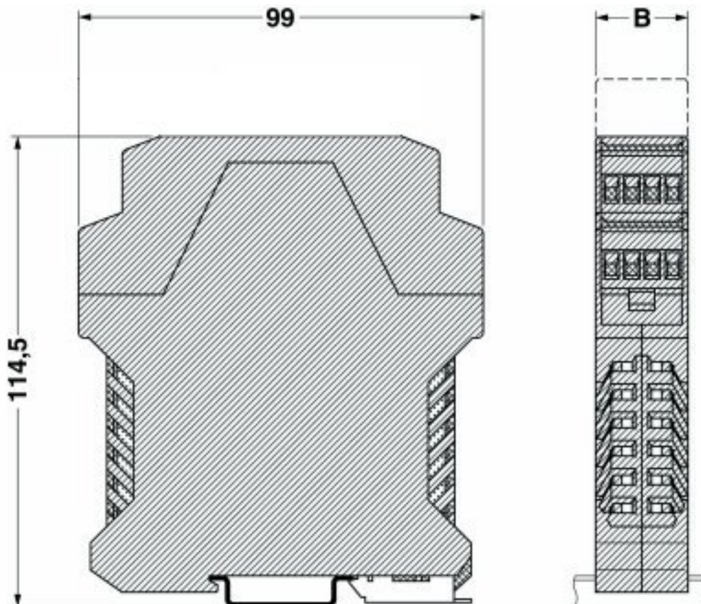
Dimensioned drawing
