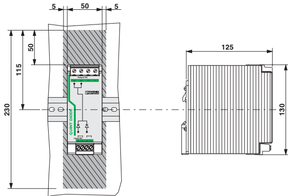
Figure 3 Installation dimensions
