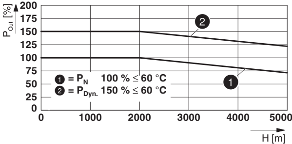
Figure 20 Output power depending on the installation height
