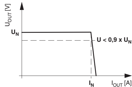
Figure 16 U/I characteristic curve
