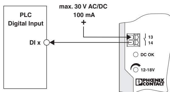
Figure 18 Wiring principle
