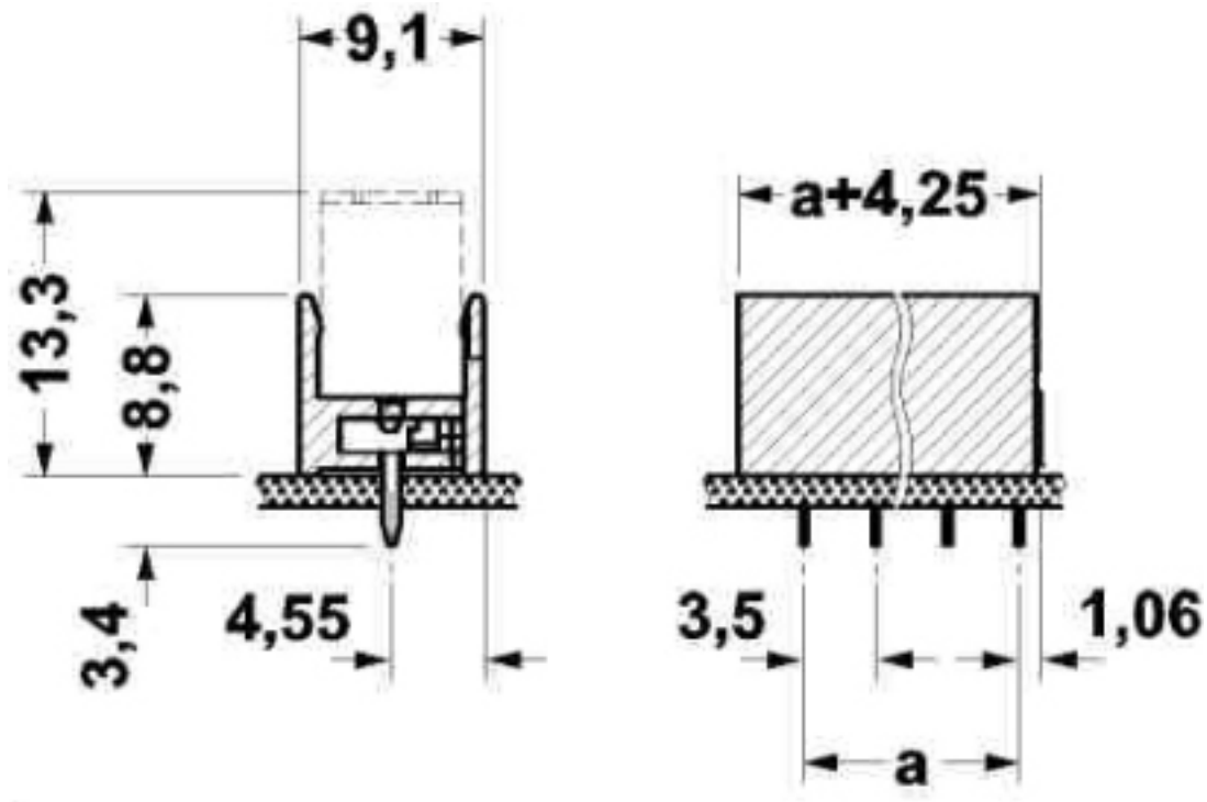
Dimensioned drawing
