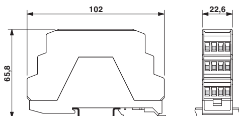
Housing dimensions, electronic housing ME 22.5 super-flat... with triple-level upper part
