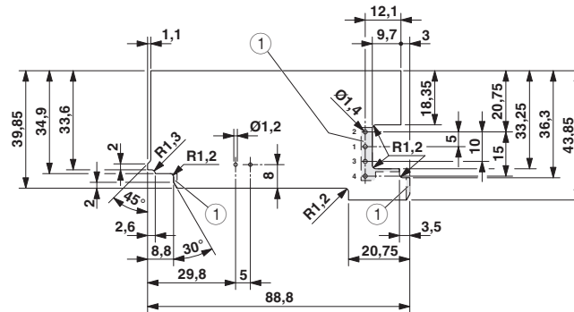
Dimensioned drawing
