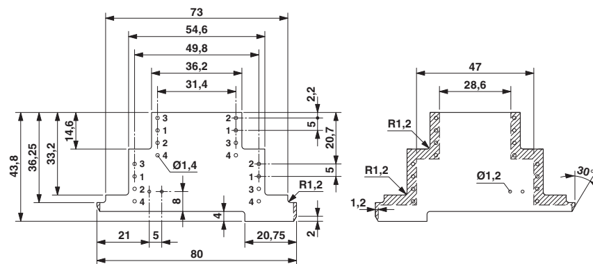
Dimensioned drawing
