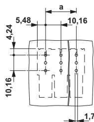
Drilling diagram
